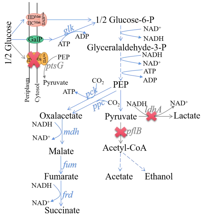
Figure S2 Central metabolic pathway of E. coli for succinate production in this work. PEP: phosphoenolpyruvate. Dashed lines represent multi-step reactions. Gene deletions are indicated in gray and crossed out.
