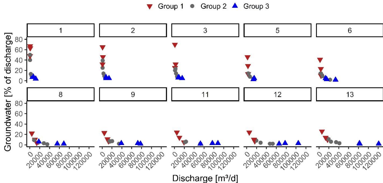
Supplementary Figure 1. Groundwater Flux as % of the total discharge for each reach. This figure shows the same data as figure 6 (B) in the main text but is divided into the reaches. In this way, it can be shown that the effect of rising groundwater proportion with declining discharge is no artifact of the discharge increasing over the stream length.
