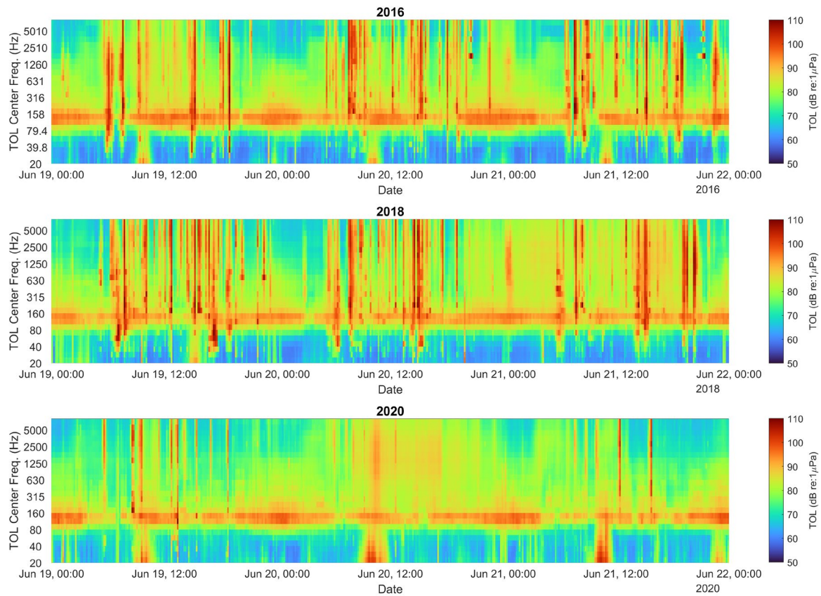
Supplemental Figure 2. One-third octave (TOL) long term spectral average plot for June 19-22 in 2016, 2018 and 2020. At this scale, individual noise events are visible including numerous vessel passages. The sound energy from harbour seal vocalizations is visible as the nearly continuous horizontal signal between 79.4 and 158 Hz. The periodic red energy at low frequencies (<39.8 Hz) is caused by tidal flow over the hydrophone sensor.
