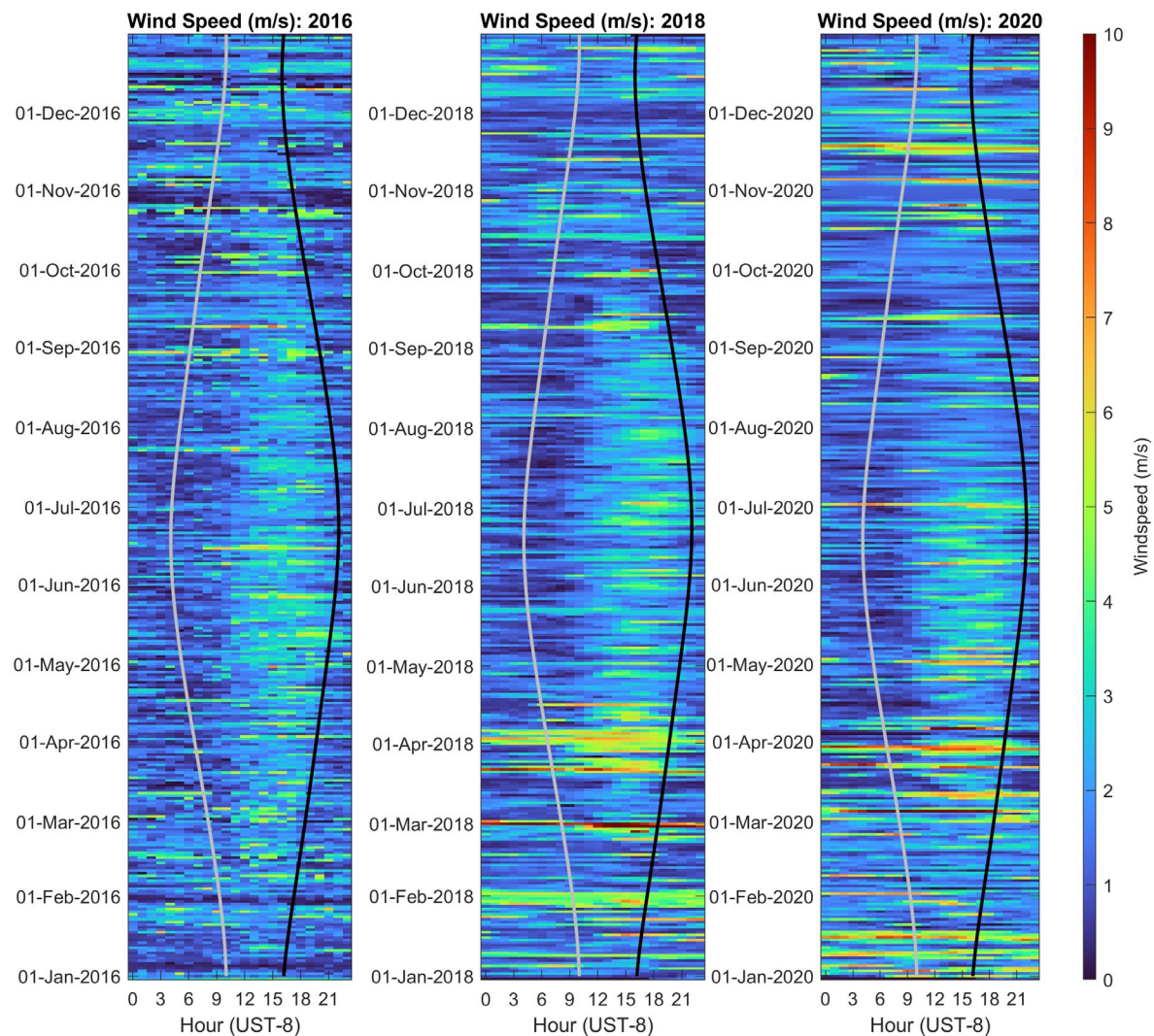
Supplemental Figure 3. Hourly wind speed data in Glacier Bay for 2016, 2018 and 2020 with wind speed indicated according to the color scale at right. Wind creates surface disturbances that result in wave, turbulence, droplet and bubble activity that create ‘wind noise’, long recognized as a primary source of underwater noise. Intense wind events (storms) are shown in yellow and red. The predominant summer wind pattern of increasing afternoon westerly or south-westerly winds is also evident. The light gray line indicates sunrise time and the black line indicates sunset time.
