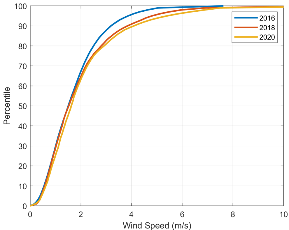
Supplemental Figure 5. Cumulative distribution of wind speeds in lower Glacier Bay in May-September 2016, 2018 and 2020. Wind speeds are based on data from DarkSky API in 2016 and from the NOAA National Data Buoy Center station BLTA2 in Bartlett Cove in 2018 and 2020.
