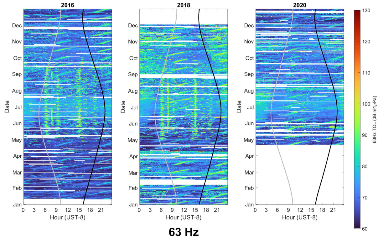
Supplemental Figure 1. Spectral density for the 63.1 Hz one-third octave band in lower Glacier Bay. The 63 Hz band is considered a standard metric for documenting the effect of shipping traffic on the underwater sound environment. The light gray line indicates sunrise time and the black line indicates sunset time. Spectral density plots for all one-third octave bands (8.91-8910 Hz) in 2016, 2018 and 2020 are compiled in Video 1 .
