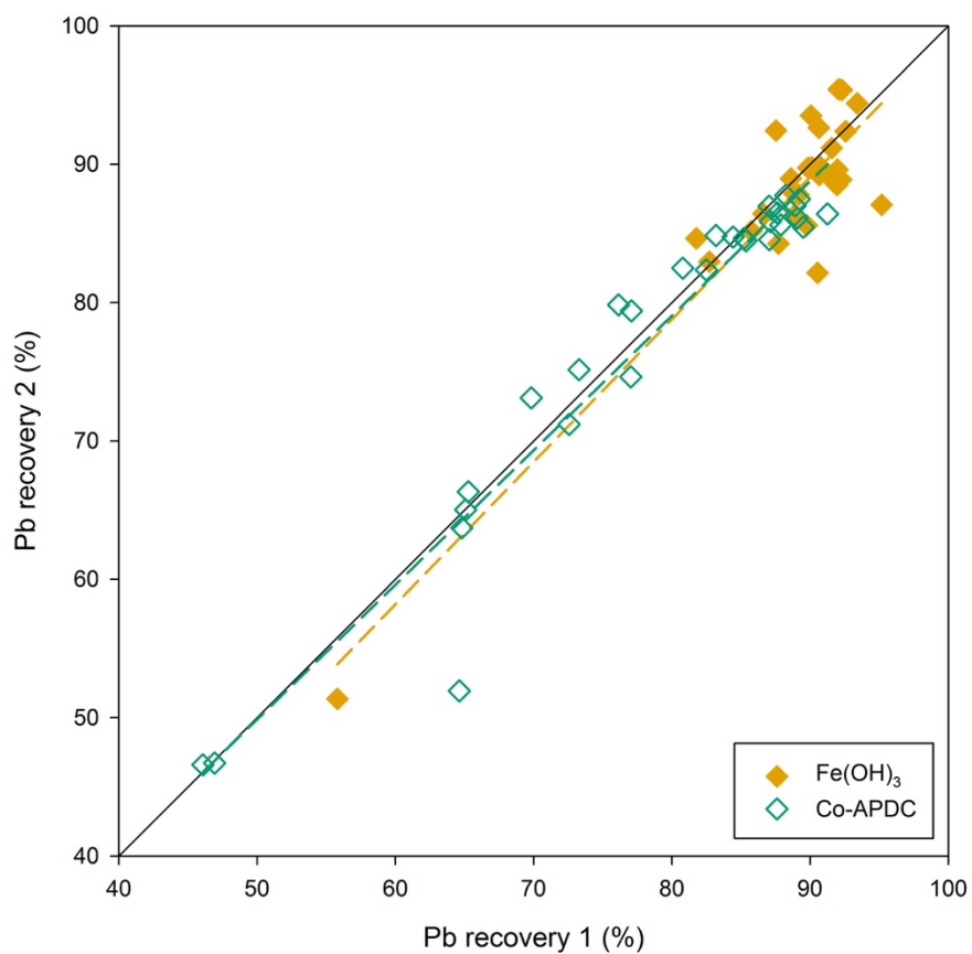
Figure S1: Recovery of stable lead at the last versus the first plating for samples processed using the \text{Fe}(\text{OH})_3 (yellow, closed symbols) and Co-APDC (green, open symbols) methods (see section “Duplicate Profiles of ^{210}\text{Pb} and ^{210}\text{Po} ”). Solid line indicates 1:1 relationship, and the dashed lines show the linear regressions for each method.
