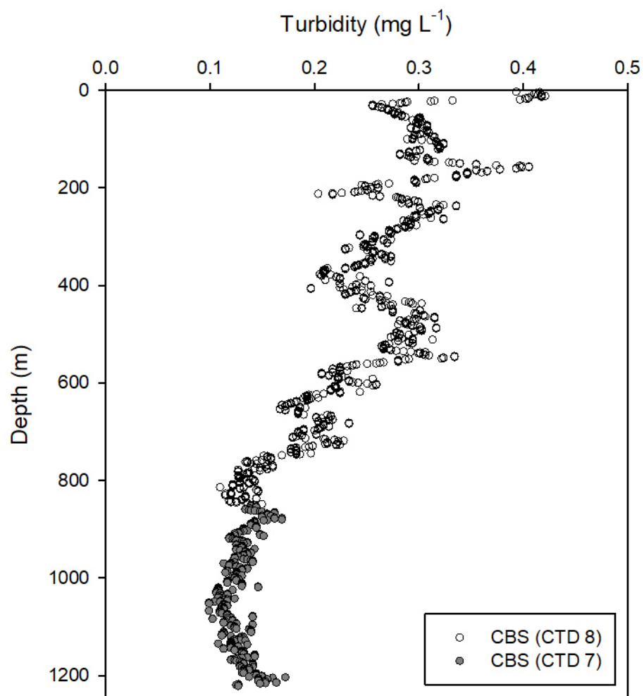
Figure S2: Turbidity profile at Catalano-Balear South (CBS) measured using a Seapoint Turbidity Sensor during two conductivity-temperature-depth (CTD) casts (7–8) from which 210 Pb and 210 Po samples were collected.
