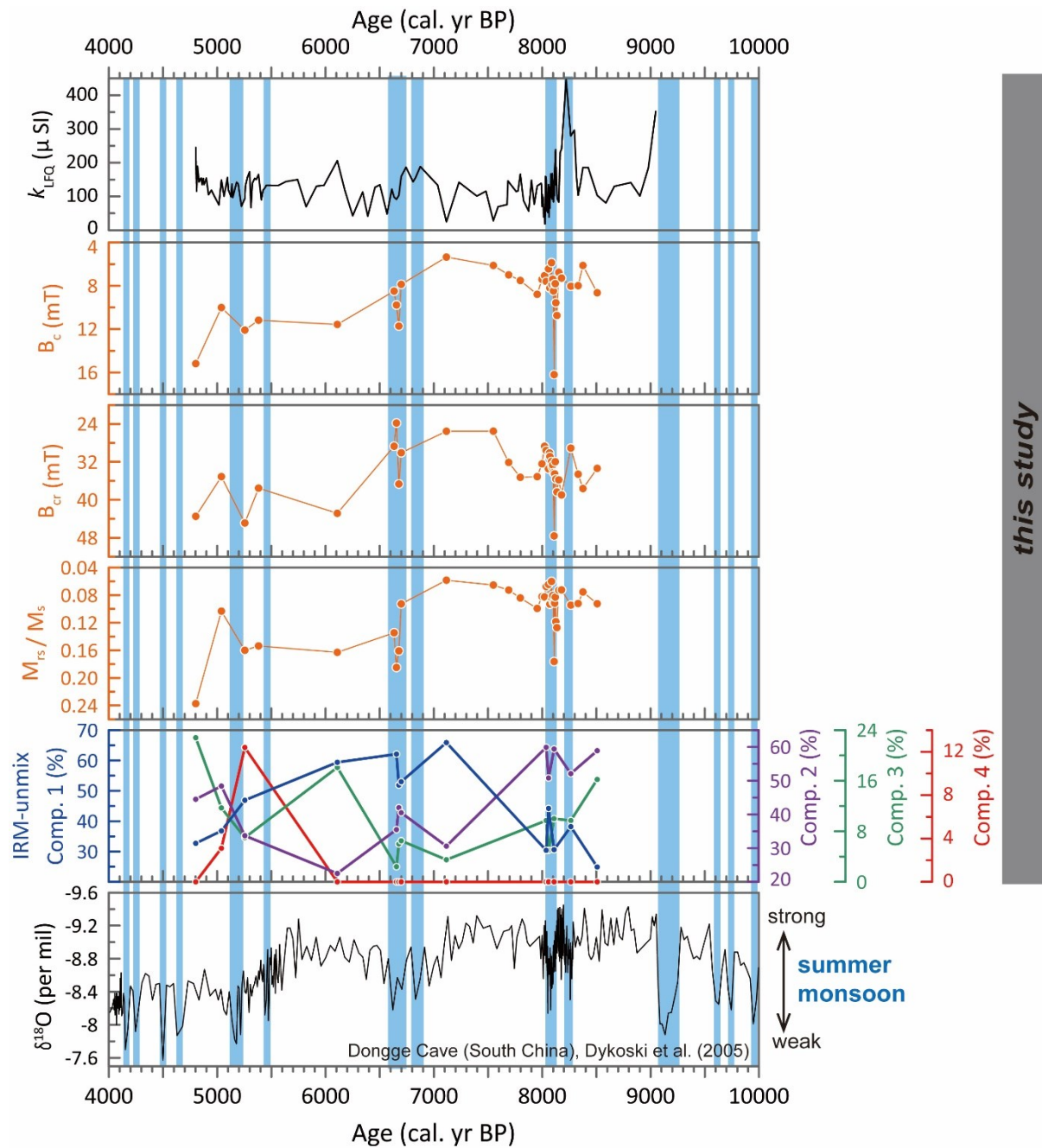
Figure S3. Comparisons between stalagmite \delta^{18}\text{O} from Dongge Cave (Dykoski et al., 2005) as a summer EAM index and some selective magnetic properties presented in this study (see text for details). Unusual high-magnitude short-term (centennial) excursions to high \delta^{18}\text{O} values indicating weak summer monsoon are indicated by blue shading.
