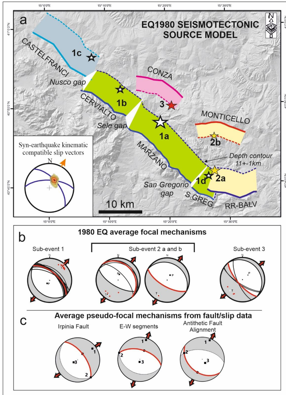
Figure S6. Box representation of the 3D seismotectonic model of Figure 12 in the main text. (A) Fault detailed segmentation pattern and link with sub-events and seismic episodes characterizing 1980 EQ. (B) Average focal mechanisms of the sub-event 1 (0 to 18 sec), sub-event 2 (20 sec) and sub-event 3 (40 sec from a compilation of data in the literature resumed in Table S3 and in Figure 2A . (C) Pseudo focal mechanism derived from data represented in the stereoplots of Figure 5A .
