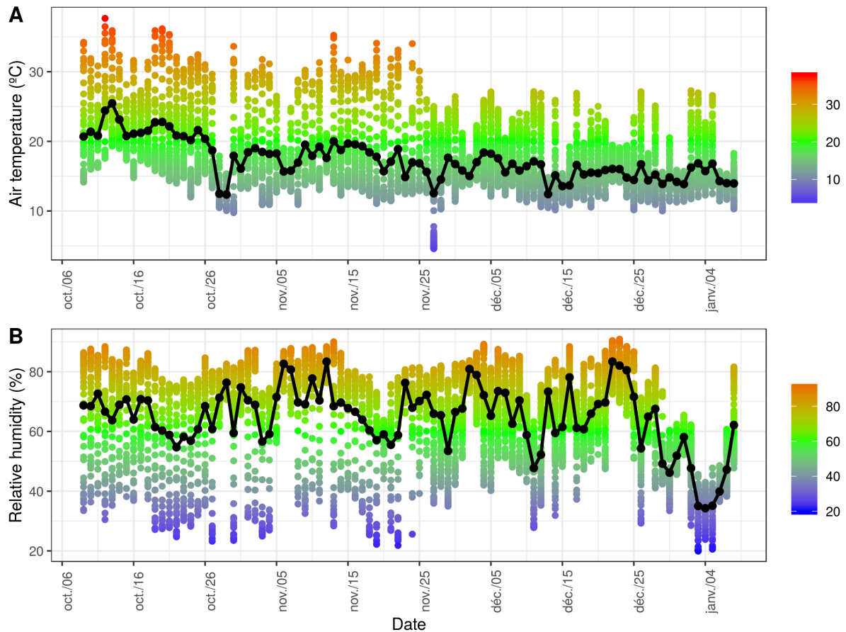
Figure S1. Plant growth conditions in the greenhouse. Air temperature (A) and relative humidity (B) during the experiment. For each measurement mean is shown in black line.
