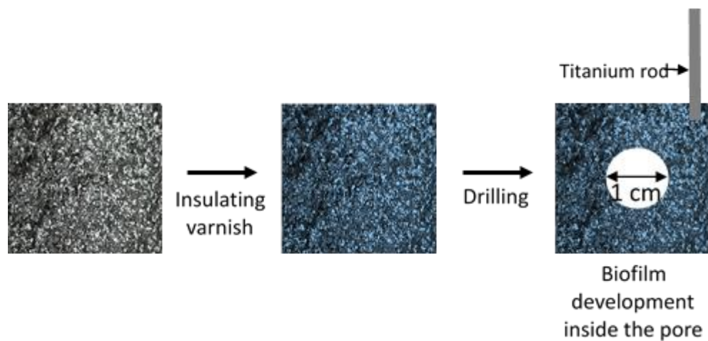
Supplementary Figure 2: Graphite electrodes preparation strategy for internal biofilm development
