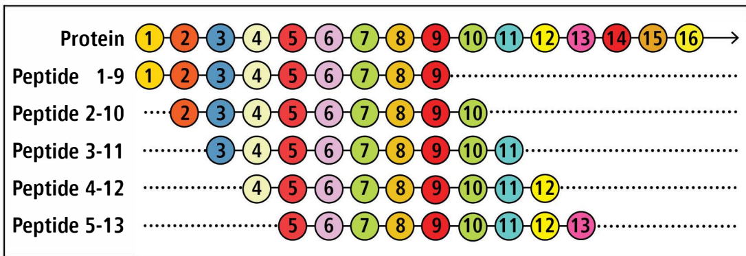
Supplementary Figure 4. Illustration of the 9-mer peptide library used for brute force epitope mapping of HCMV pp65. The first sixteen positions of the pp65 amino acid sequence are shown on the top. The individual peptides walk the sequence in steps of single amino acids.
