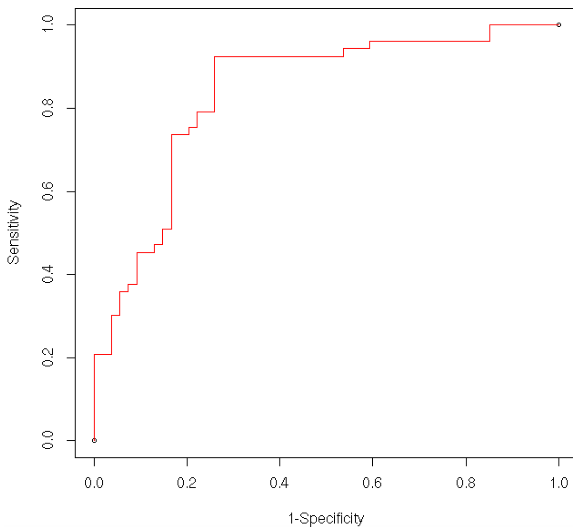
Figure 2: ROC Curve of multivariate model to discriminate NP from NNP
