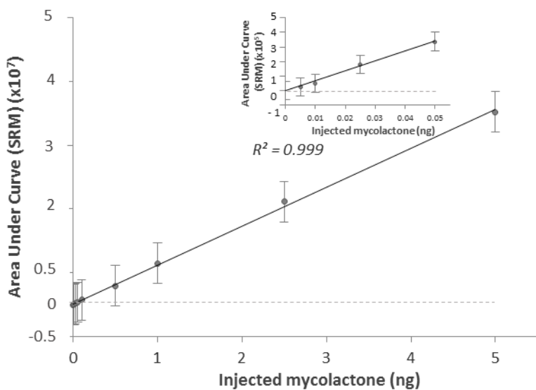
Supplementary figure 1: Detection and quantification of mycolactone by liquid chromatography coupled to tandem mass spectrometry
