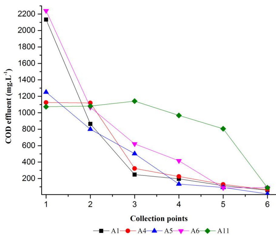
Figure S1. Degradation of organic matter along the reactor 1 (R1).
