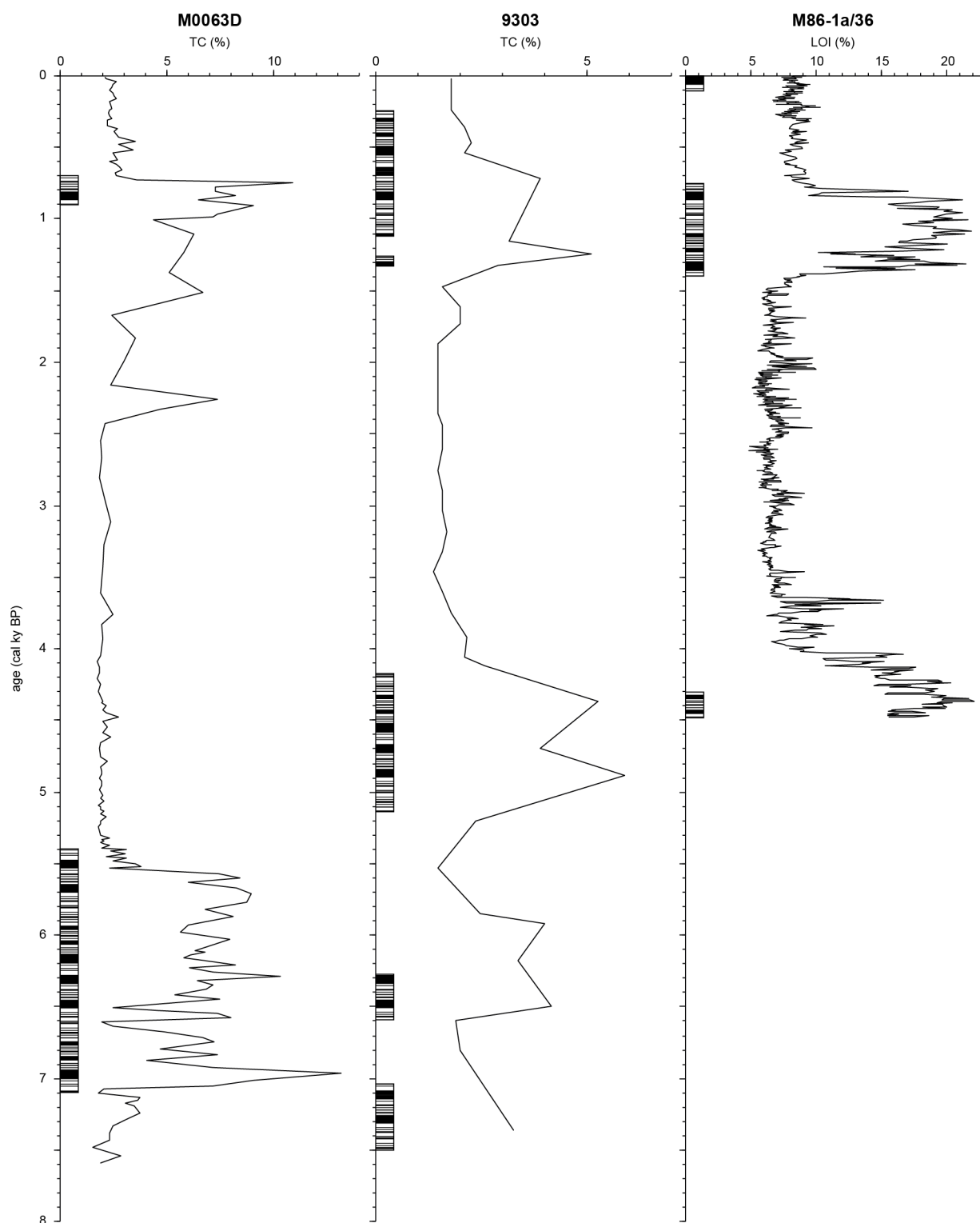
Supplementary Figure 2. Total carbon content (%) and prominent laminated sequences of Integrated Ocean Drilling Program Expedition 347 core M0063D (This study), core 9303 (Bianchi et al., 2000) and core M86-1a/36 (Häusler et al., 2017) plotted versus calibrated ages (cal ky BP).
