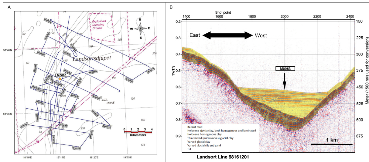
Supplementary Figure 1. A) Track plot of seismic survey lines in the Landsort Deep around Site M0063 (yellow diamond). Distance between isobaths is 100 m. ODAS = Oceanographic Data Acquisition Systems. B) Close-up of transect along seismic Line 68161201, crossing Site M0063, with original interpretation of seismic signals. TWT = two-way travelttime. Figure from Andren et al., 2015.
