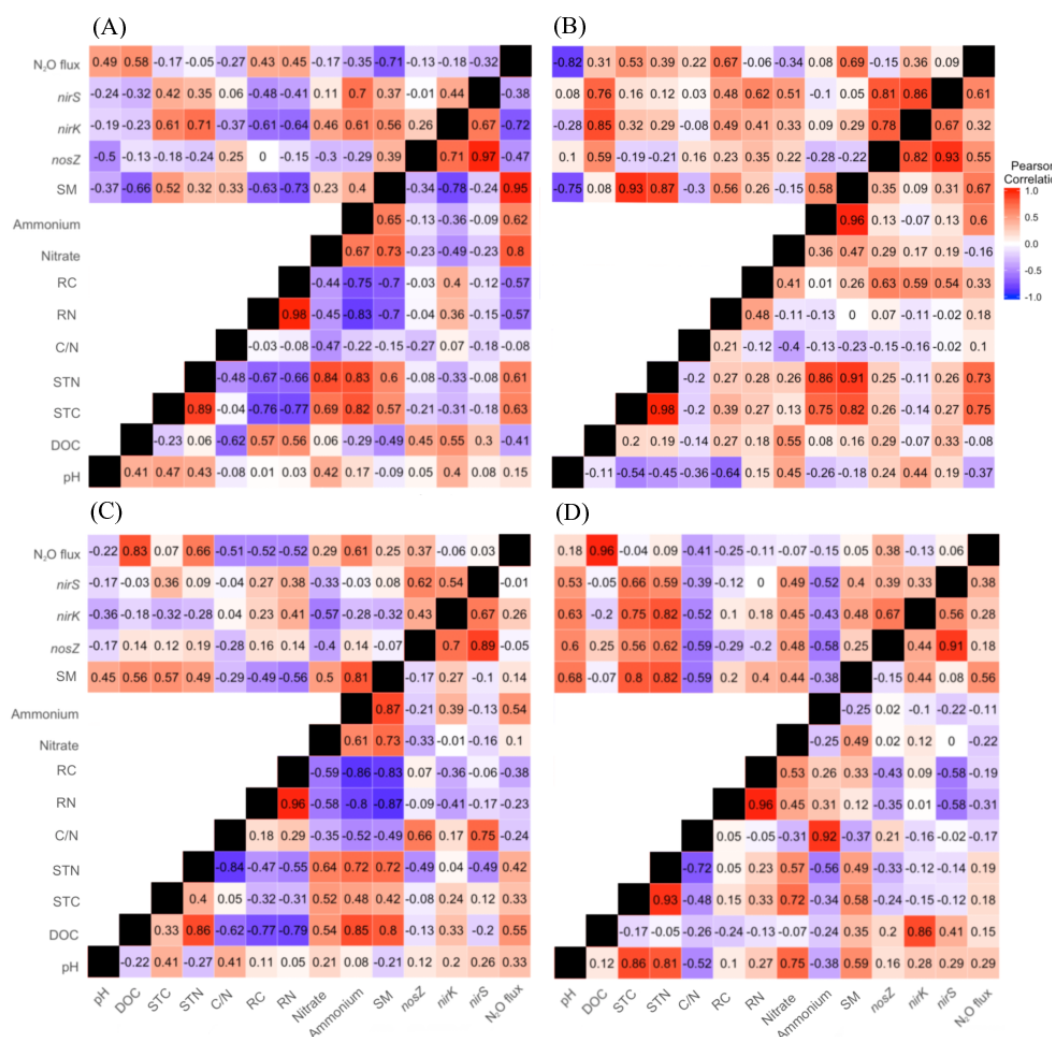
Supplementary Figure 2. Pearson correlations determined to evaluate the relationships between the soil chemical, physical and genetic variables. The heatmap color and text indicate the correlation coefficient. The data from the field are presented in the lower triangle, and data from the soil incubation experiment are presented in the upper triangle. The data are from the (A) Citrus; (B) Forest 1; (C) Eucalyptus; and (D) Forest 2 sites from the field (lower right-hand triangle) and incubation experiments (upper left-hand triangle). The soil moisture data were derived from field moisture (not controlled incubation moisture) for both triangles; C/N from soil total C and N.
