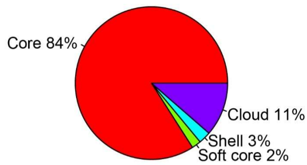
Supplementary Figure 3 | Proportion of different types of genes in the pangenome of 147 M. tuberculosis genomes.
