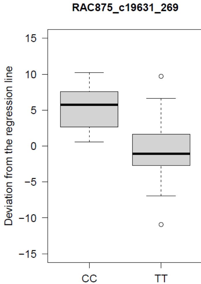
Suppl. figure 7: Boxplots of genotype means for the deviation from the regression line based on number of kernels per ear for genotypes with the CC or TT allele at the QTL marker RAC875_c19631_269.
