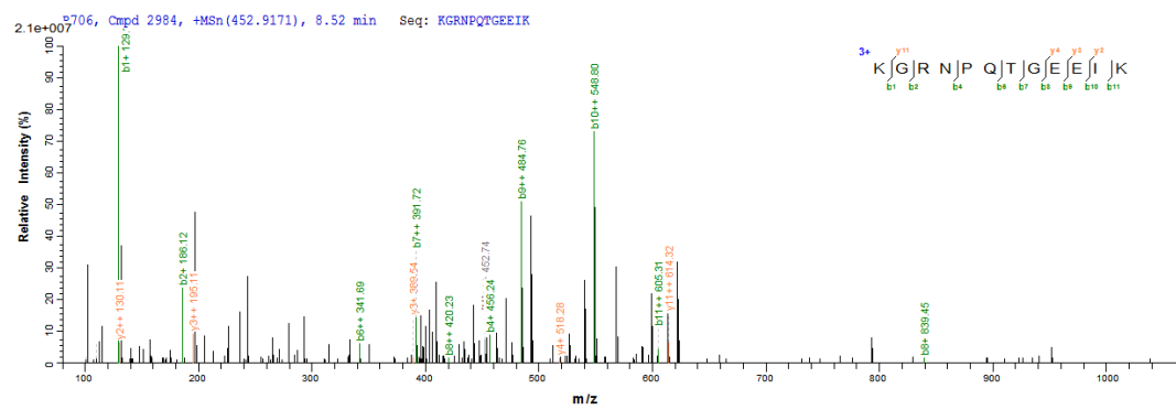
Fig. S2 Fragments of BM1122 identified by LC-MS/MS.
